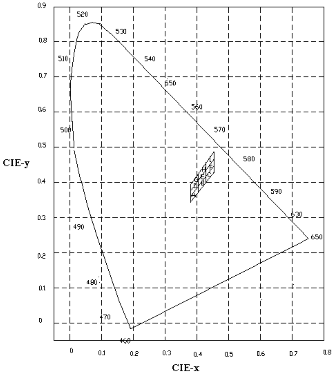
Chromaticity Coordinates Specifications for Bin Rank
